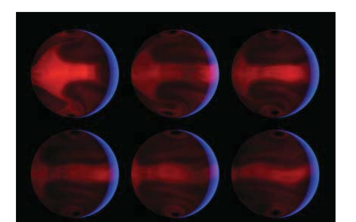
This series of temperature maps made using Spitzer Space Telescope data depicts what temperature swings an extrasolar gas giant planet HD 80606b travels in a highly elliptical orbit around its star. Bright areas are hottest.
